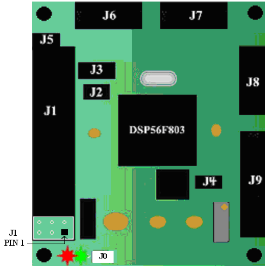
Figure 1 – Connector J1
